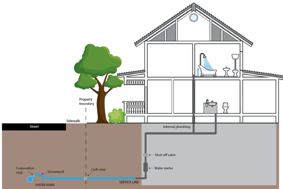
Graphic of Water Service Line Connection from Water Main in Street to Building
